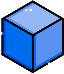
Cube
