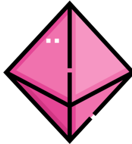
Octahedron
