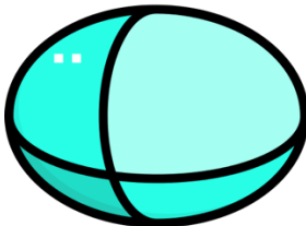
Ellipsoid
