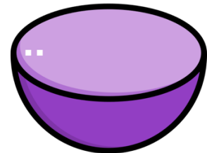
Hemisphere
