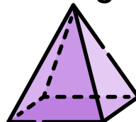
Square Pyramid
