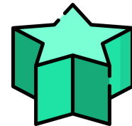
Pentagrammic Prism
