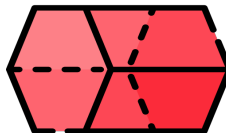
Hexagonal Prism
