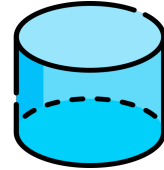
Cylinder
