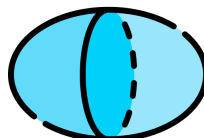
Ellipsoid
